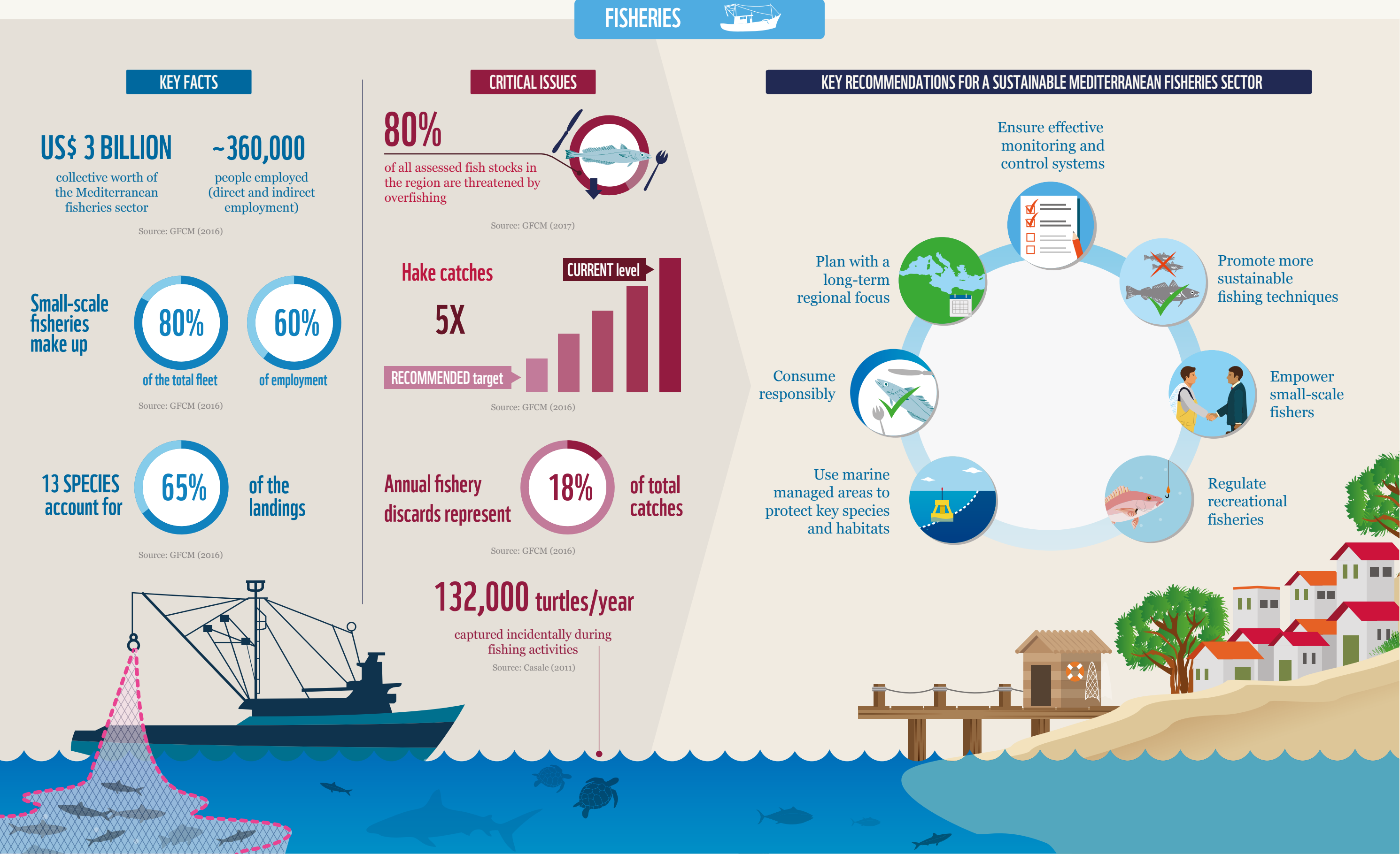
FIGURE 6 MEDITERRANEAN FISHERIES: STATE AND RECOMMENDATIONS
